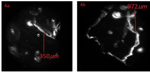
Figure 4: Longest microcrack lengths measured for (a) control group, and (b) gamma ray 26-30 kGy emission range group. Both microcrack lengths concerning the case of 32-year-old samples.
