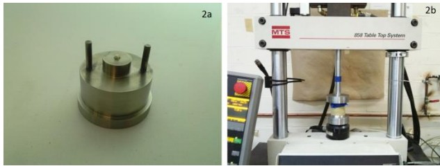
Figure 2: (a) A cortical human bone sample placed in the custom-made mounting, before performance of the fatigue compression tests; (b) Cortical human bone sample placed in the custom-made mounting, during the fatigue tests.
