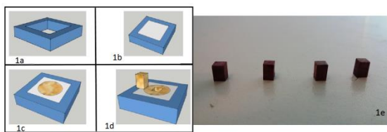
Figure 1: Machining and staining process of cortical bone samples. (a) Image of stainless steel frame; (b) Addition of plaster and water mixture before the integration of bone segments; (c) Integration of bone segments in the plaster and water mixture; (d) With the use of a CNC machine, cortical samples were extracted from the plaster and water mixture to be subjected to fatigue compression tests; (e) Samples of cortical segments of human femurs, after being stained with alizarin complexone.
